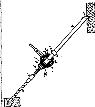
24331 Willard's Rock and Coal Drill.
