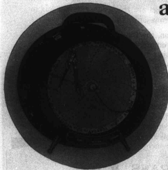
Bristol's Portable Thermo-Humidigraph, Model 4069. Eight inch chart. Specify Model 4068 for surface mounting in permanent location. Charts for 24 hour or 7 day records. Model 4044 four inch Humidigraph, with-out pen arm for recording temperature, also available.
