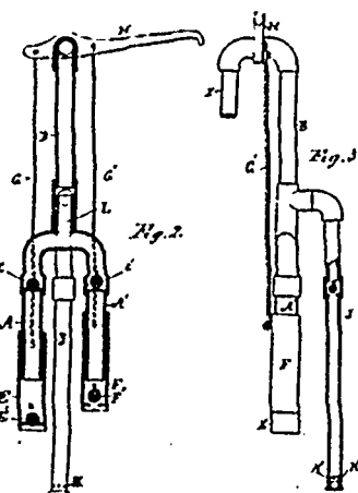
28494 Clark's Lift Pump
