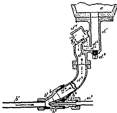
28496 Gresham's Apparatus for Applying Sand to the Driving Wheels of Locomotives.
