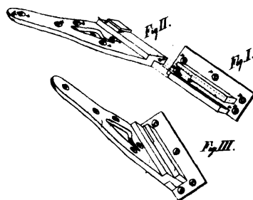
8960 Chevigny's Bedstead Fastening.
