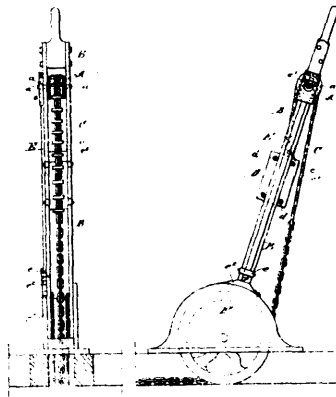
39582 Doorey, Minehan, Lodge, Boniface and Allen's Compensator for Signal Rods.
