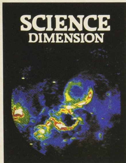
DRAO
