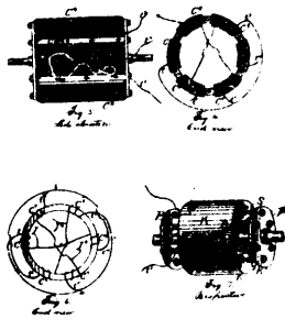
12331 Thomson & Houston's Improvements on Armatures for Dynamo-electric Machines.
