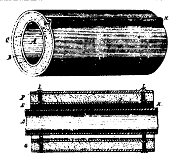
12339 Battelle's Improvements on Coverings for Pipes, &c.
