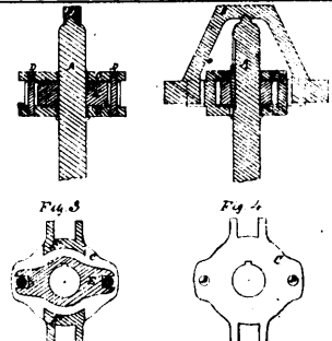
12332 Bogart & Mitton's Improvements on Millstone Drivers.
