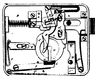
12340 Russell's Improvements on Indicator Locks.
