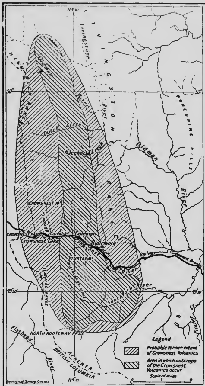
Figure 1. Diagram showing location of the Crowsnest volcanics.
