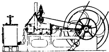
3587 Hock's Improvements on Motor Engines Worked by the Combustion of Petroleum or other Liquid Hydro-carbons.
