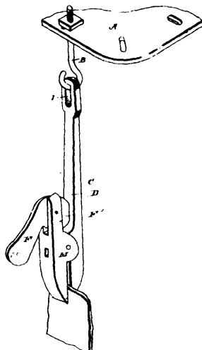
27426 Ellithorp's Clamp for Lasting Machine.
