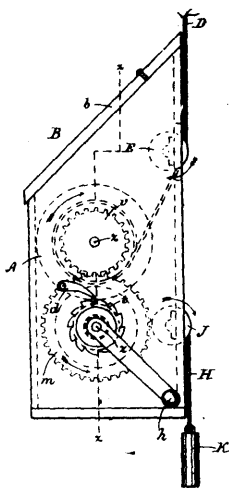
27423 Crowley &amp; Kelley's Clothes Line Reel.
