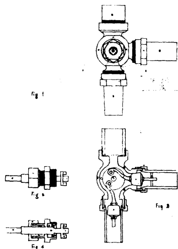
27422 Meadows' Water Closet Valve.
