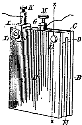
25950 Prismuth's Galvanic Cell.
