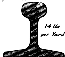
Fig. 14. Sections of Rails.
