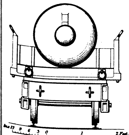
Fig. 15. End Elevation.
