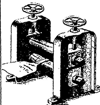
25392 Myer's Apparatus for Manufacturing Shovel Spades, etc.
