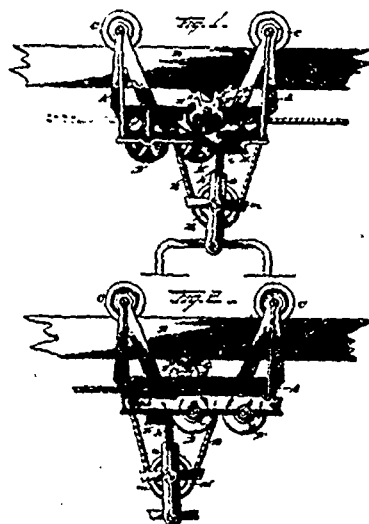
25398 Osborn's Hay Elevator.
