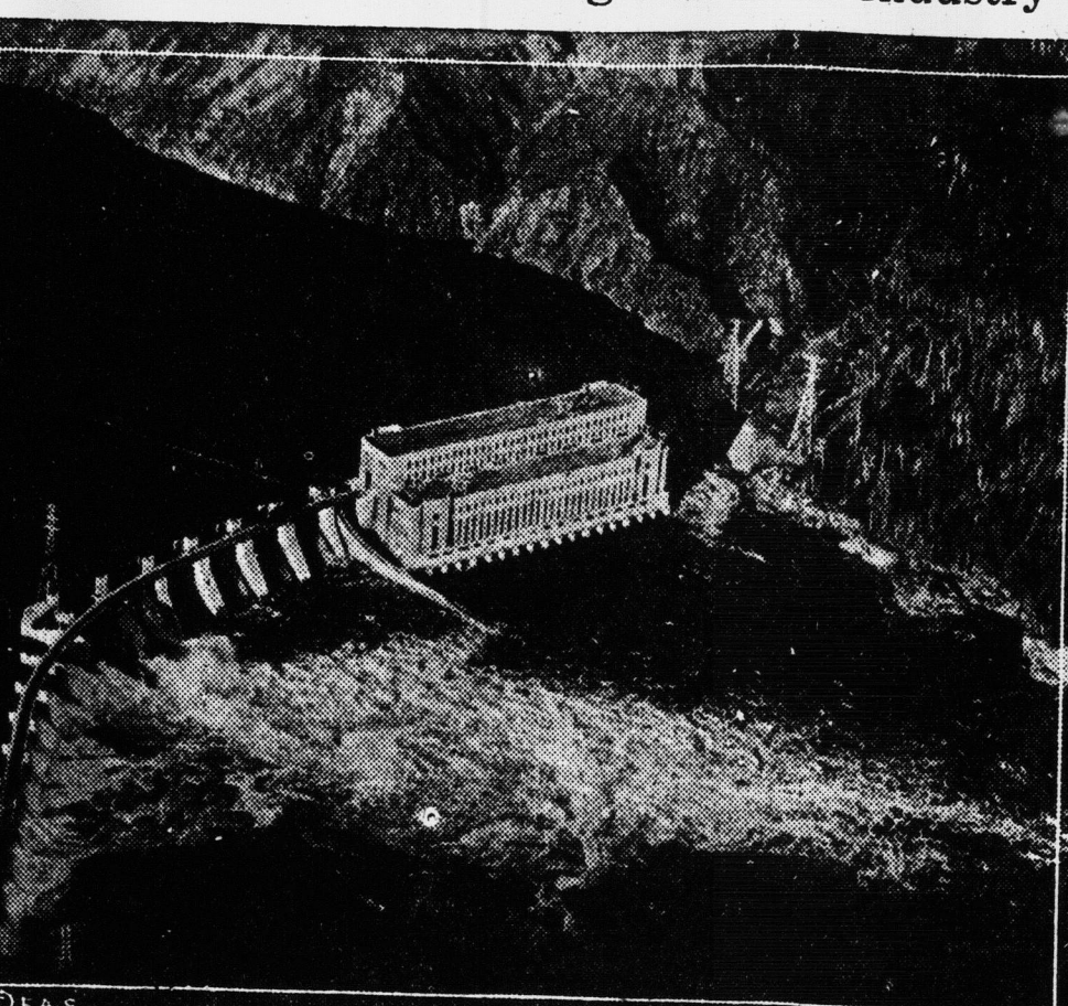
Hydro-electric power plant at La Gabelle, Quebec, where the St. Maurice river is made to give up 150,000 horse-power. The plant is the property of the Shawinigan Water & Power Co.
