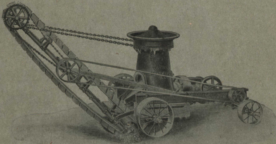
AUSTIN GYRATORY CRUSHER ON TRUCK WITH ELEVATOR.
