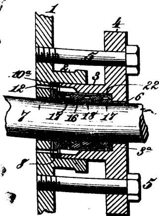
34838 Martin's Roll Packing.
