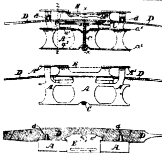
15283 Poindexter's Improvements on Saw Jointers and Gauges.
