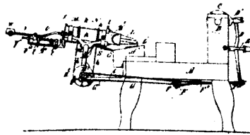
15277 Sénécal's Improvements on Automatic Feeding Apparatus for Nail Cutting Machines.
