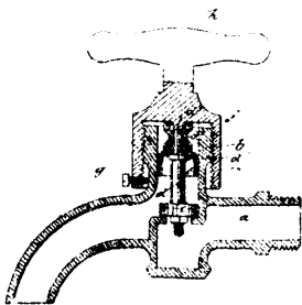
15282 Ashton &amp; Sperry's Improvements on Cocks and Valves.
