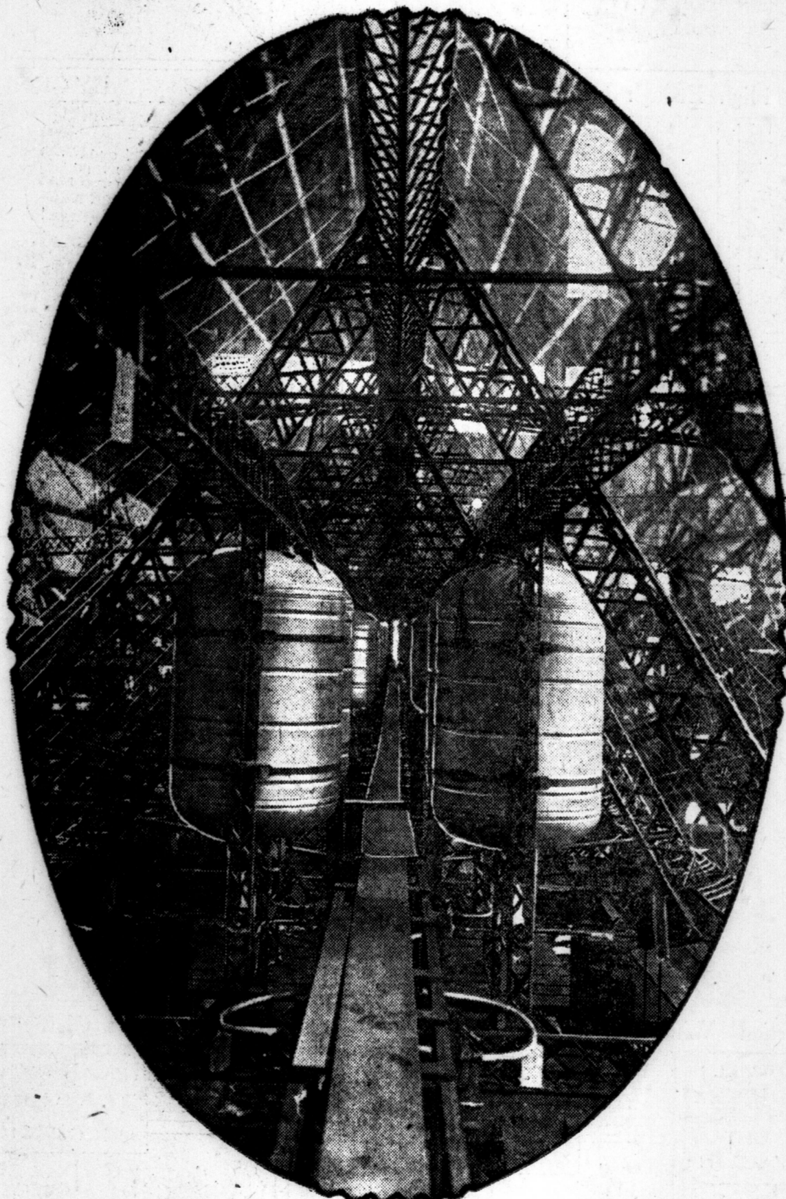
A view through the keel of the new dirigible ZR-1 showing some of the 48 gasoline tanks which hold 113 gallons each. They are built so that 16 can be slipped from the ship to lighten the weight in case of necessity.
