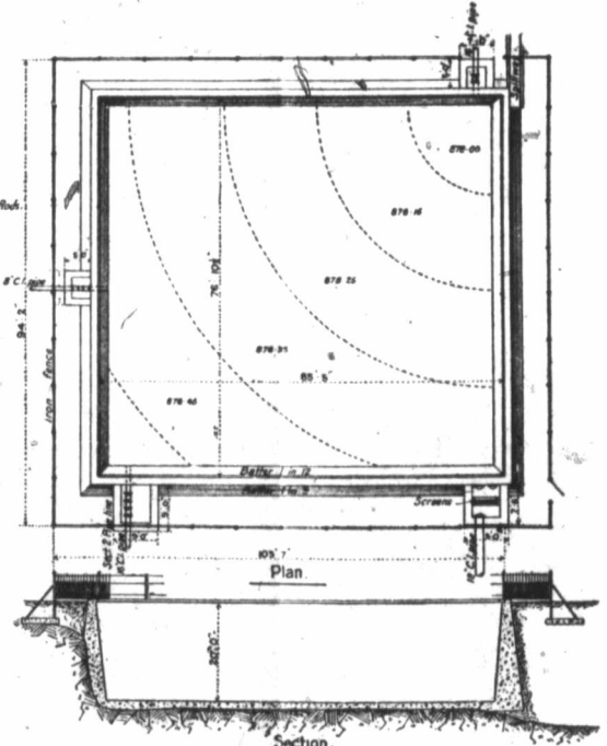
Section RESERVOIR.
