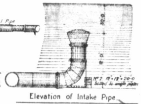
Elevation of Intake Pipe.
