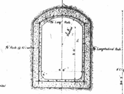
Section through Culvert connecting Gate Chamber and Tunnel.
