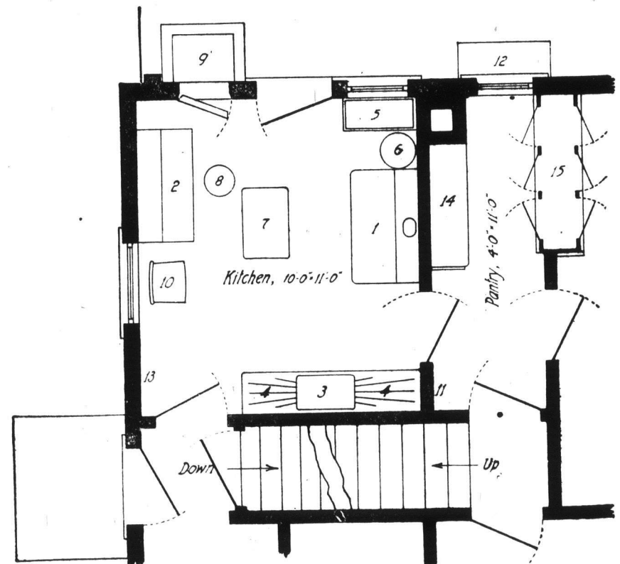
PLAN SHOWING LAYOUT OF KITCHEN
