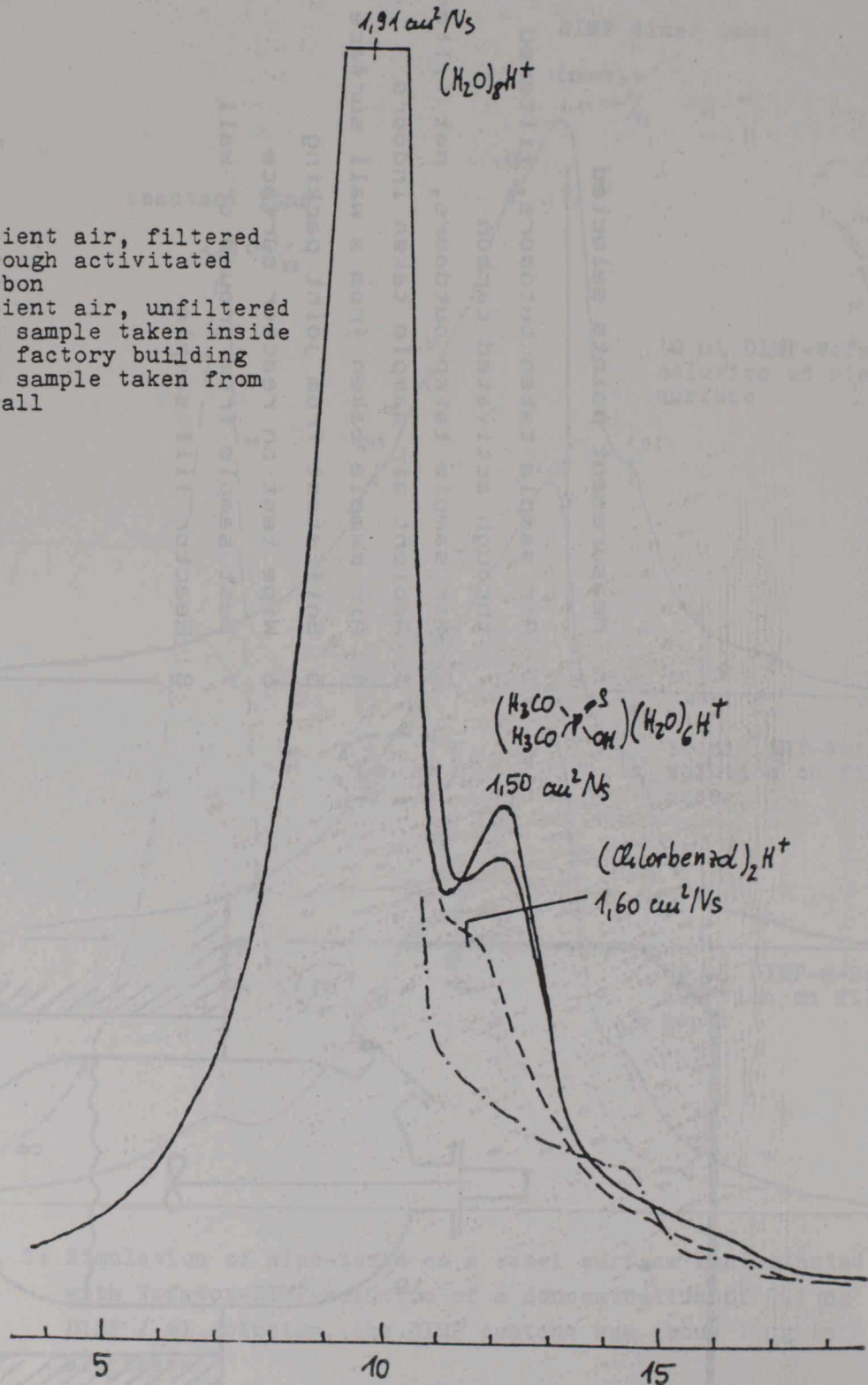
Fig. 9: IMS signals recorded at measurement points 1 to 4
