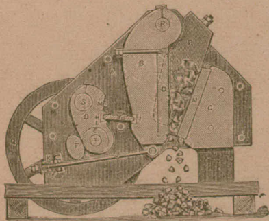
CHAMPION ROAD CRUSHER (Sectional View)
