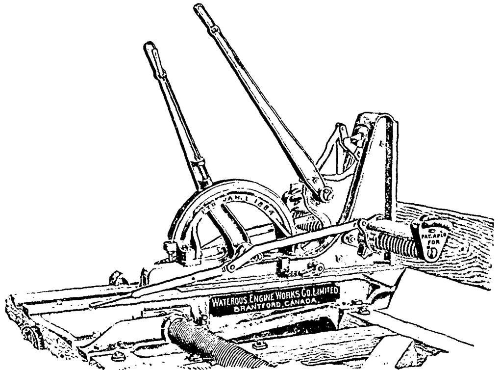
Automatic Dogging and Receding Wings.
