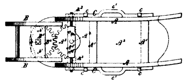
8360 Triebels & Henderson's Improvement on Coasting Sleds.
