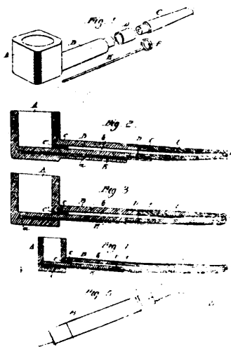
33893 Weldon's Tobacco Pipe.
