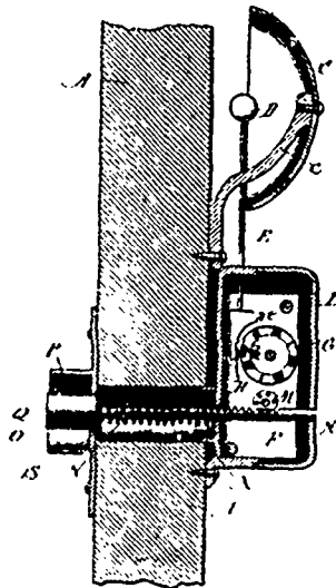
29587 Sanderson's Door Bell and Alarm.
