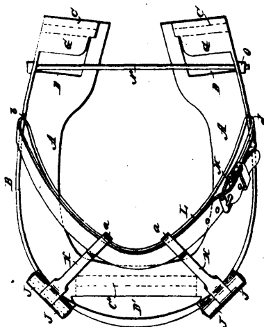
18680 Smith's Overshoe for Horses.
