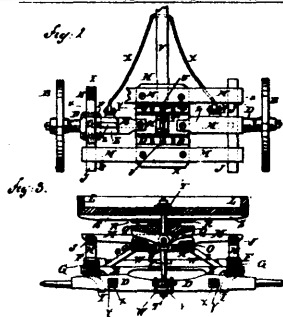
18674 Fanning's Waggon Running Gear.
