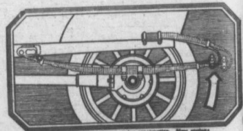
Arrows show old and new spring construction. New springs much longer and more flexible.
