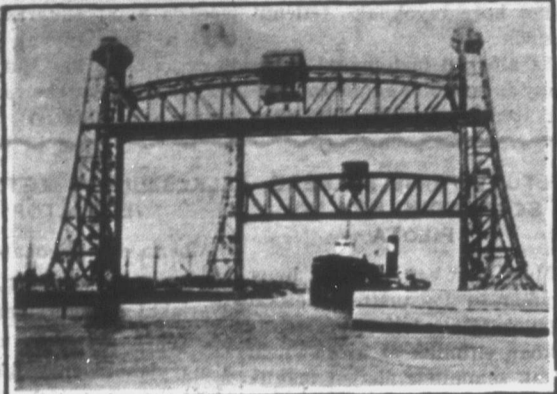
2 TYPICAL VERTICAL LIFT BRIDGES ON NEW WELLAND CANAL
