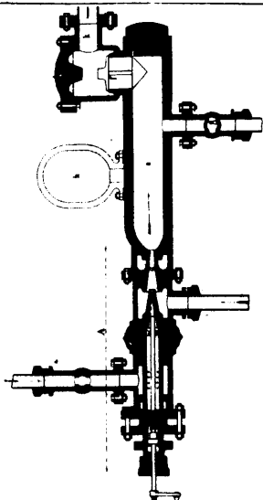
16118 Michaux &amp; Baingard's Improvement on Injectors.
