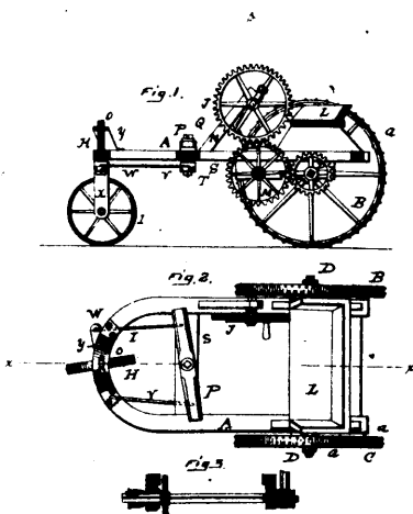
16115 Lowry's Improvements on Velocipedes.
