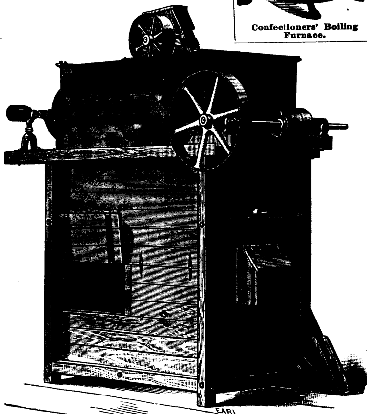
MEAD'S SUGAR MILL, WITH BOLTER AND RECEIVER.
