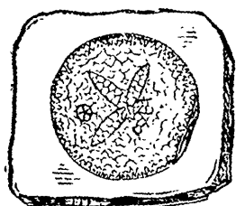
Fig. 180.— Agelacrinites Billingsii (Chapman).
