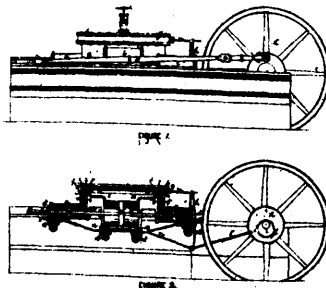
5230 Alexander's Compound Steam Engine.
