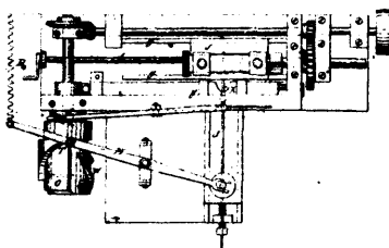
5227 Williams' Machine for Rolling Crimping Tacks, Awls, &amp;c.
