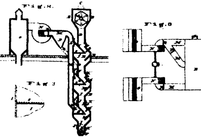
5224 Downton &amp; Miller's Middlings Purifier.
