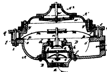
14946 Lacey's Improvements on Gas Regulators.
