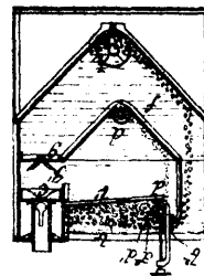
14939 Sheppard's Improvements in Coal Washing Machines.
