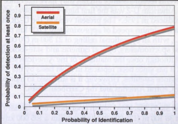
Figure A-3. Overall Detection Probability — Satellite Surveillance
