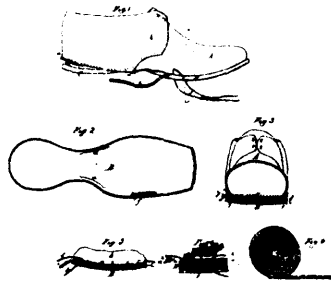
12655 Pratt's Improvement in Boots and Shoes.
