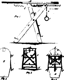
12653 Blodget's Improvements in Ironing Tables.
