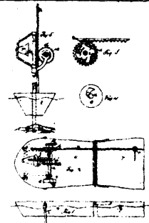
12659 Close's Improvements on Fog Signals.
