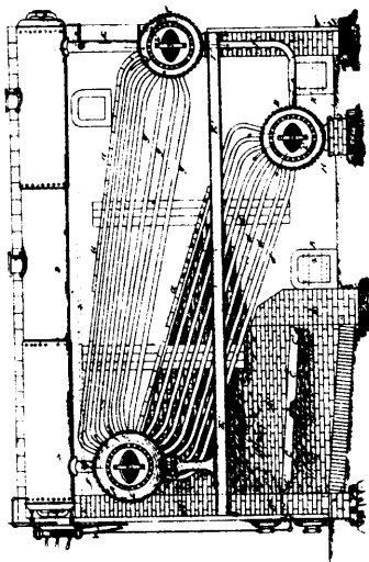
38807 Zell's Steam Boiler.
