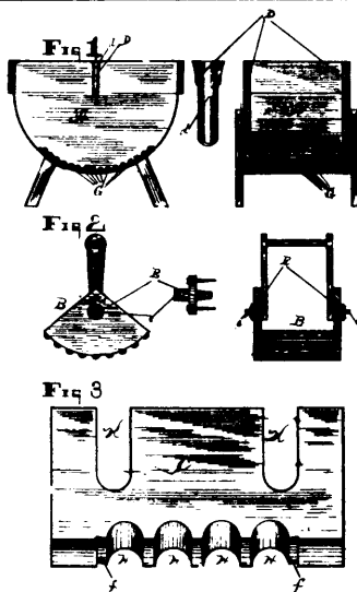
34758 Waugh's Washing Machine.
