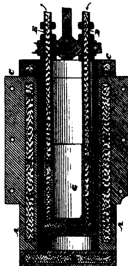
17967 Stetson's Hydro Carbon Engine.
