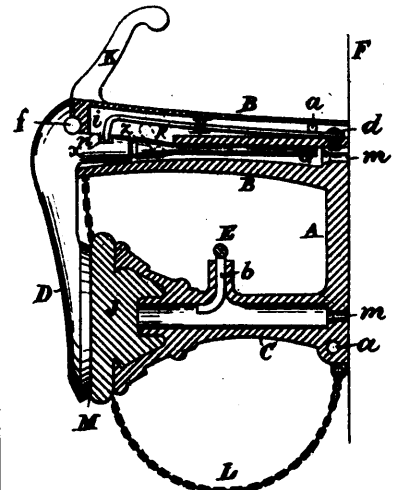
17962 Mill's Coat Hook.
