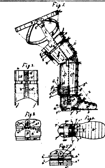
17961 Burn's Club Foot Apparatus.
