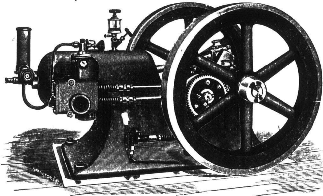
The Power that runs our Presses. 2 1/2 h. p. Gasoline Engine
