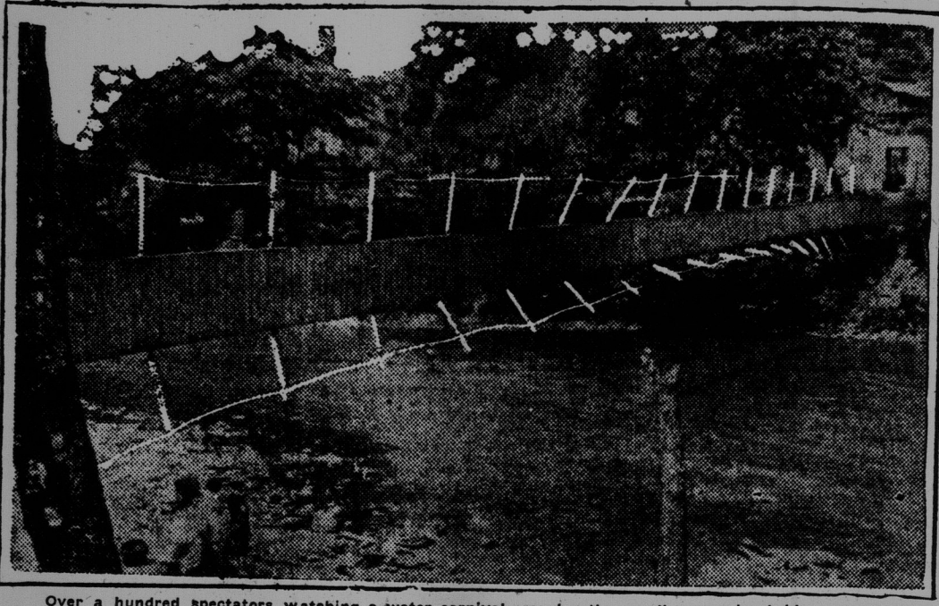
Over a hundred spectators watching a water carnival crowded the small suspension bridge over the Coal River at Whitesville, West Va. A concerted shift of the crowd from one side of the bridge to the other overstrained one of the two supporting cables, which broke. The bridge fell into the position shown in this photo and cast its occupants onto the rocks and into the water below. Six were killed and sixty injured. The photo was made just after a special train had removed the victims from the scene of the tragedy.
