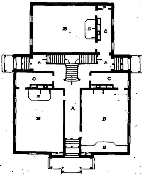
GROUND PLAN FOR TWO STORY SCHOOL HOUSE.
