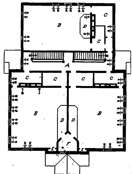
SECOND FLOOR FOR TWO STORY SCHOOL HOUSE.
