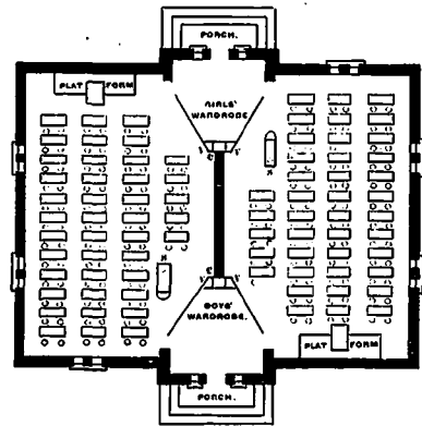
GROUND PLAN FOR A GRADED, RURAL, OR VILLAGE SCHOOL.
