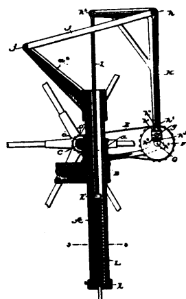
40105 Althouse's Windmill.
