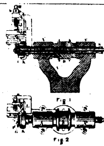
7929 Busell's Machine for Preparing the Edges of Soles.
