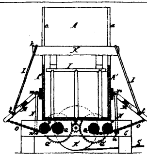
14825 Herring's Improvements in Baling Presses.
