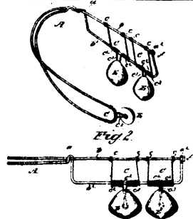
14821 Herrick's Improvement in Trusses.
