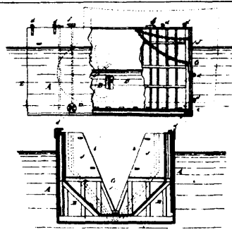
14826 Kirkham's Improvements in Coffor Dams.
