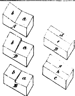
14818 Dupuis's Improvements in Bricks.
