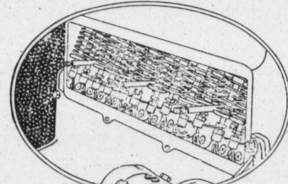
Light-Six valves are inclined at a 20-degree angle, which position increases power and contributes unusual quietness of operation.
