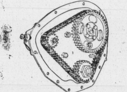
Silent chain, running in a constant spray of oil, takes the place of the usual timing gears, and thereby contributes to the quietness of the Light-Six motor.
