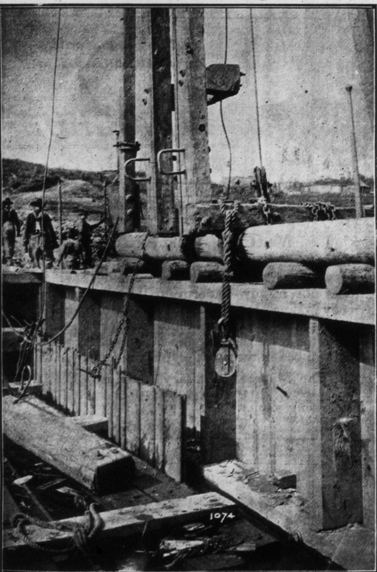
WITH THE BUILDERS OF DAMS. The big coffer-dam at Abitibi River during construction. Piles were driven deep into the soft river bottom, in order to secure solid foundations.
