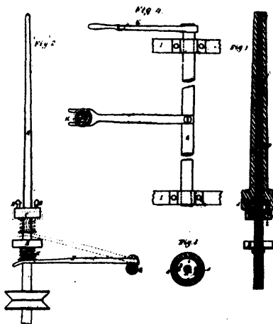
22650 Cuthbertson's Spinning Machine.
