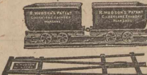
38—Pass-by, with Fixed Points Castings only
