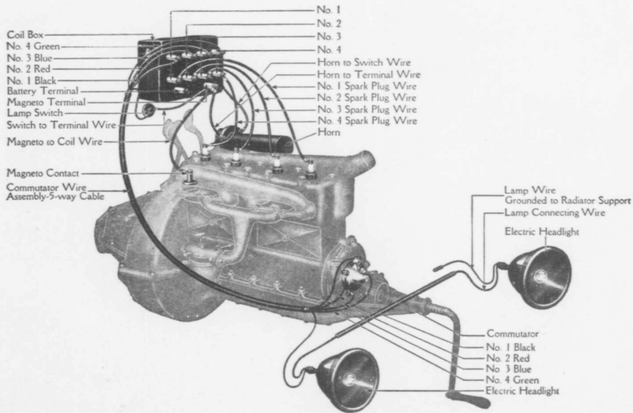
Wiring of the Ford Ignition System, also Electric Horn and Headlamps. (Cut No. 11)
